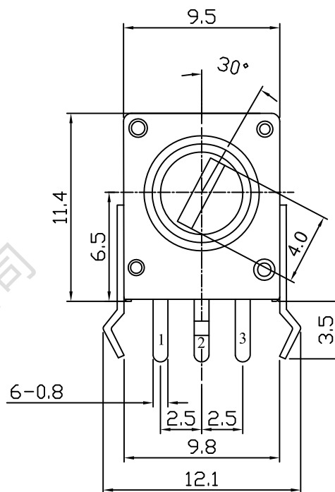
Shaft shown in full C.C.W. position
